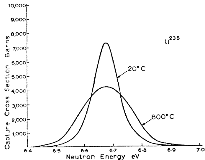
Fig. 2 Doppler Broadening
